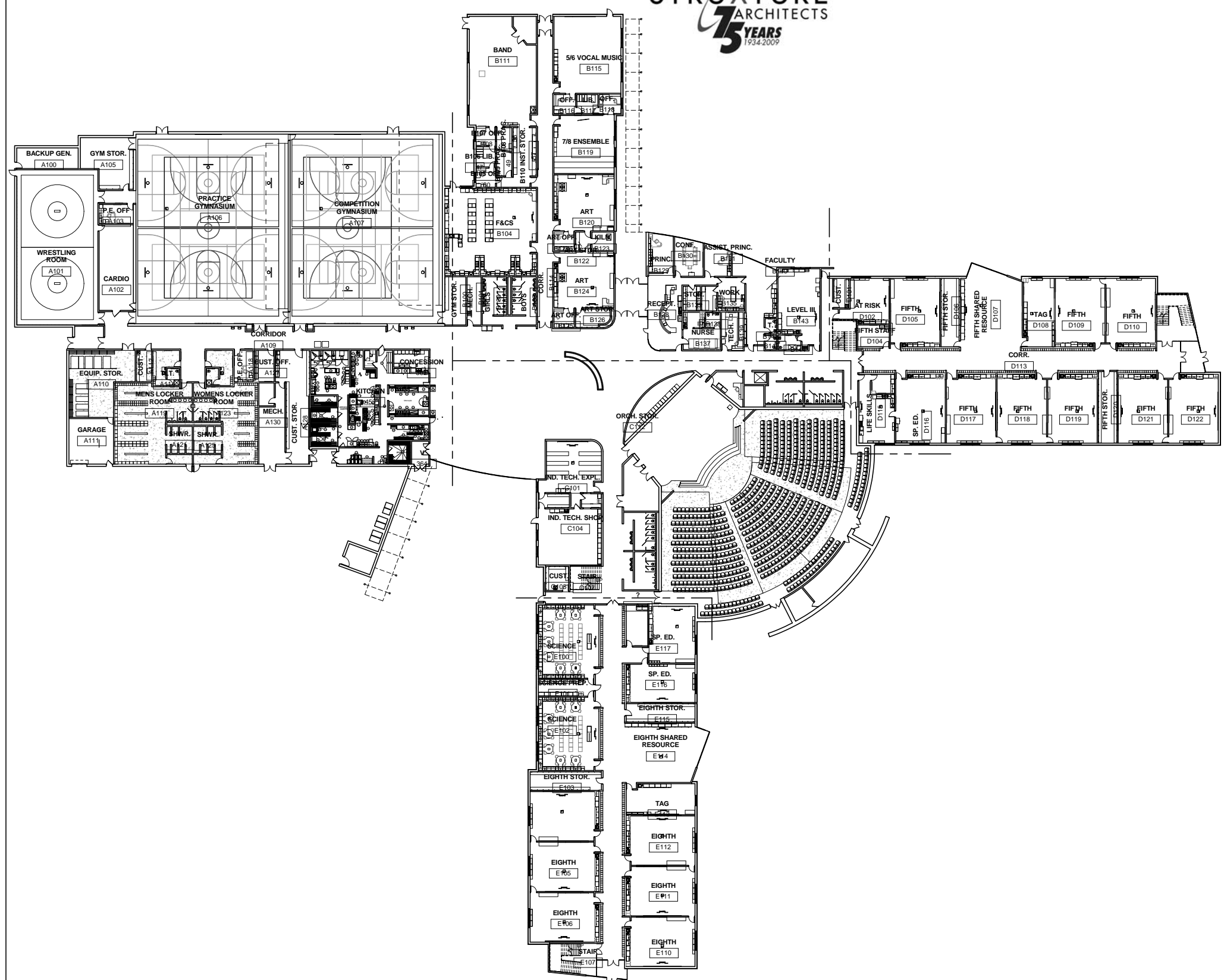
OVERALL FIRST FLOOR 1" = 20'
